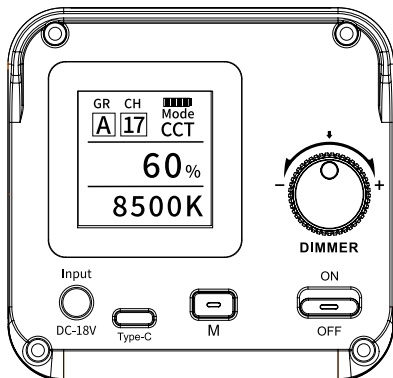
Operation Interface
